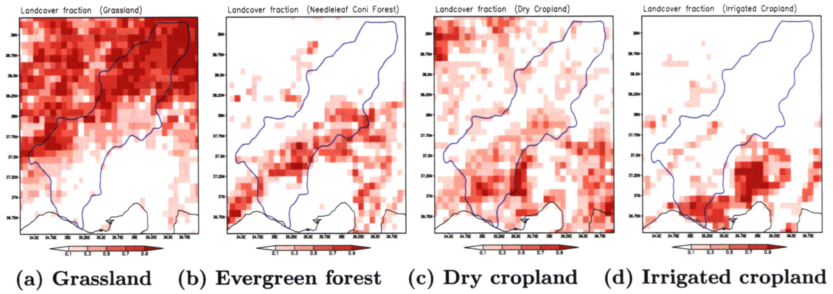
Fig. 3 : Landcover fraction of each grid (5 min resolution)
