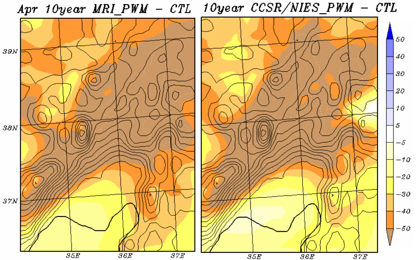
Fig. 11. Horizontal distribution of difference in precipitation between present and future climate in the finest grid downscaled form MRI-CGCM (left) and CCSR/NIES-CGCM (right)
