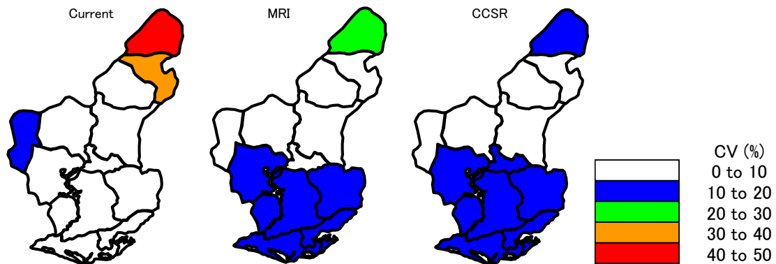
Fig. 7. Coefficients of variation in year-to-year change of wheat yield in Adana (predicted by SimWinc).
