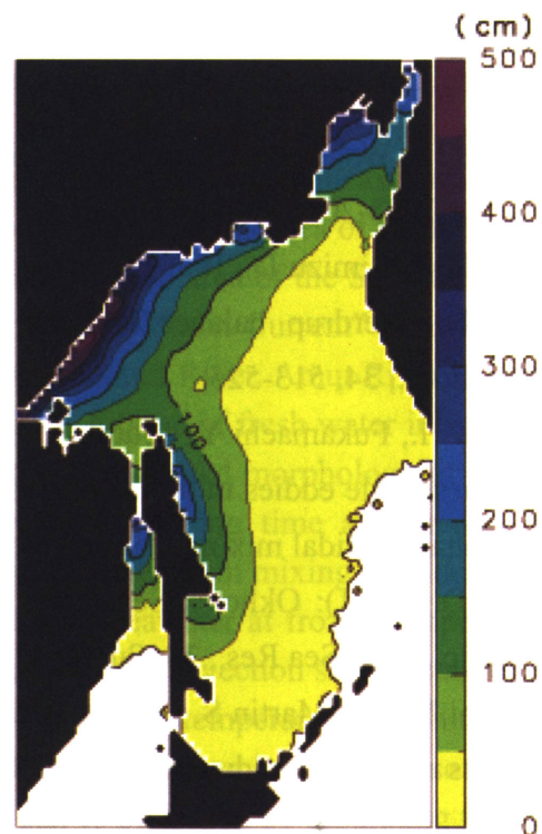
Figure 9: Spatial distribution of annual cumulative ice production (represented by the ice thickness: cm) averaged over 1987-2001. (Ohshima et al., 2003)
