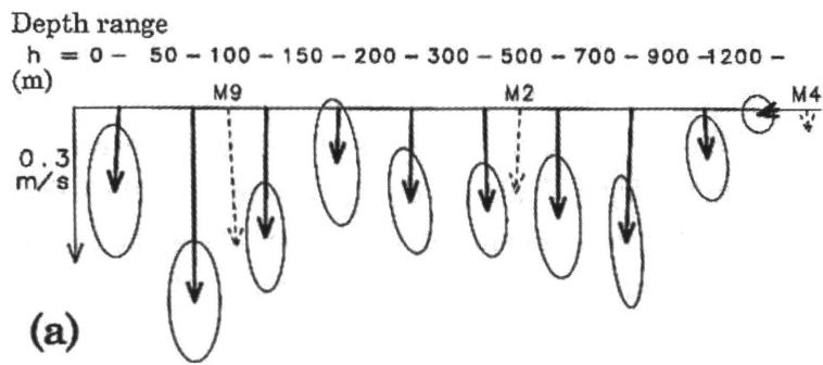
Figure 2. Mean velocity vectors as a function of bottom depth range with a coordinate aligned with the depth contour direction for 51.5-55°N in the East Sakhalin Current region. The associated 95 percent confidence error ellipses are also shown at the tip of the vectors. Mean velocity vectors from the moorings are also shown by dashed lines. (Ohshima et al., 2002)
