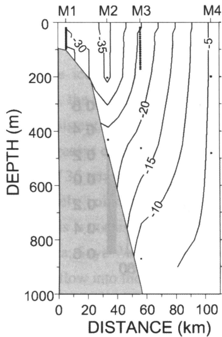
Figure 5: Monthly mean velocity component ( \text{cm s}^{-1} ) normal to a vertical cross section at 53^\circ\text{N} in January 1999. Positive value indicates a southward flow. (Mizuta et al., 2003)
