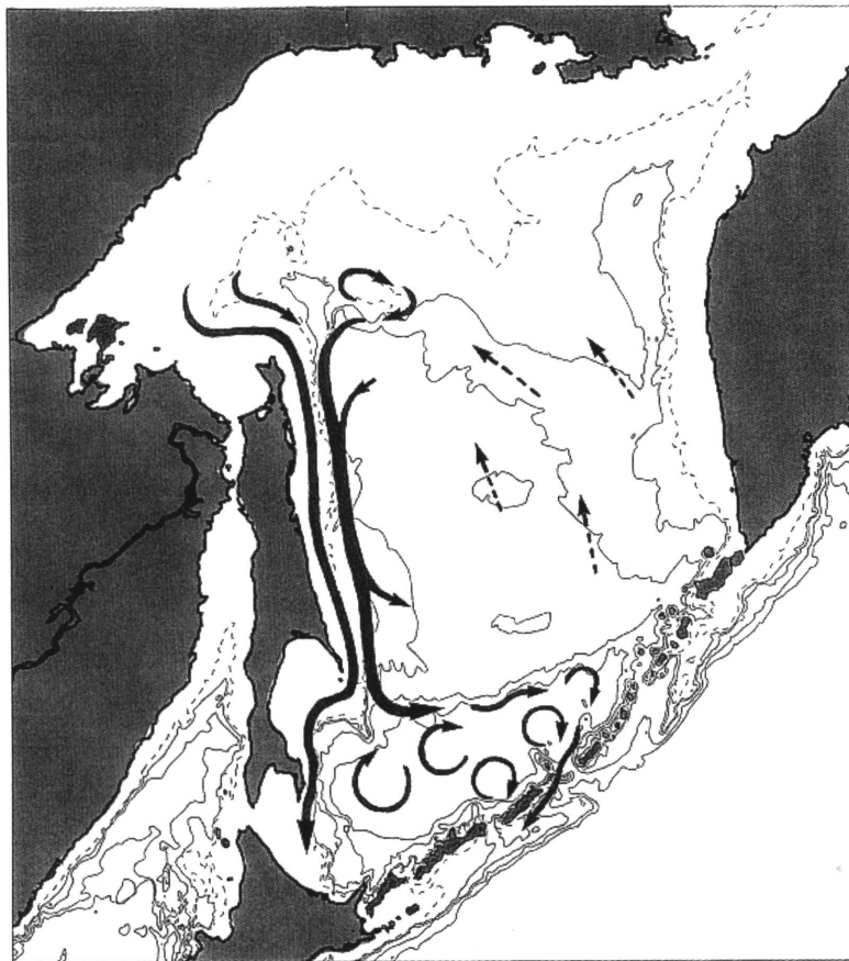
Figure 3: Schematic of near-surface circulation for the Sea of Okhotsk as derived from our satellite-tracked drifter data. Thicker arrows represent the stronger flow. Currents in the eastern part are depicted by dotted lines because they are based on speculation.
