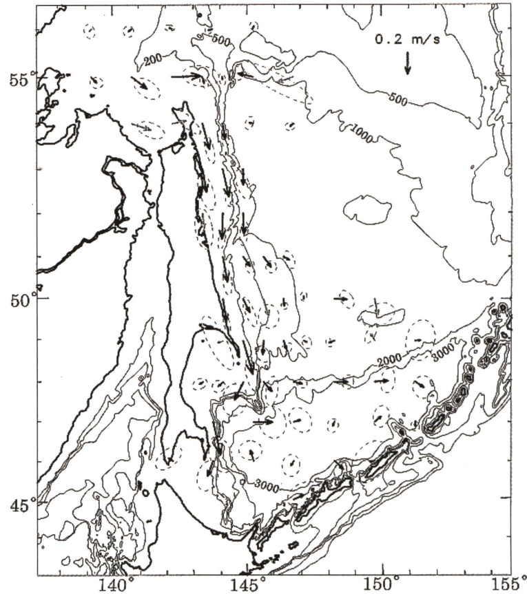
Figure 1: Mean velocity vectors for 1.5^\circ longitude \times 1^\circ latitude bin derived from 20 surface drifters. The results for bins with less than 3 drifter-days are not shown and those with less than 10 drifter-days are indicated by gray arrows. The 95 percent confidence error ellipses are also drawn around the tip of the vectors. (Ohshima et al., 2002)
