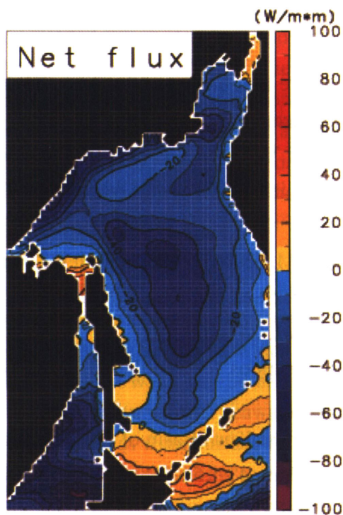
Figure 8: Annual mean net heat flux during 1987-2001. A positive value indicates that the sea (or sea ice) gains heat from the air. Areas with negative values are dotted. The contour interval is 10 \text{ W m}^{-2} . (Ohshima et al., 2003)
