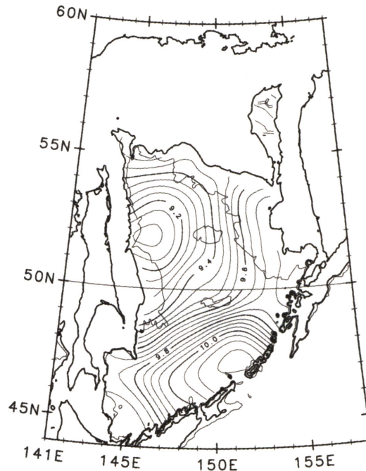
Figure 4: A chart of geopotential anomaly of 100-dbar surface relative to 1000-dbar surface in dynamic meter \times 10. The contour interval is 0.05 in dynamic meter \times 10. For the value of geopotential anomaly in the area shallower than the reference level of 1000 dbar, the extrapolation is made. (Ohshima et al., 2004)
