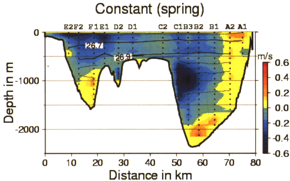
Figure 7: Mean components of the long-channel flow at the spring tide across the Bussol' Strait. The positive sign indicates the flow toward the Okhotsk, into the paper. (Katsumata et al., 2004)
