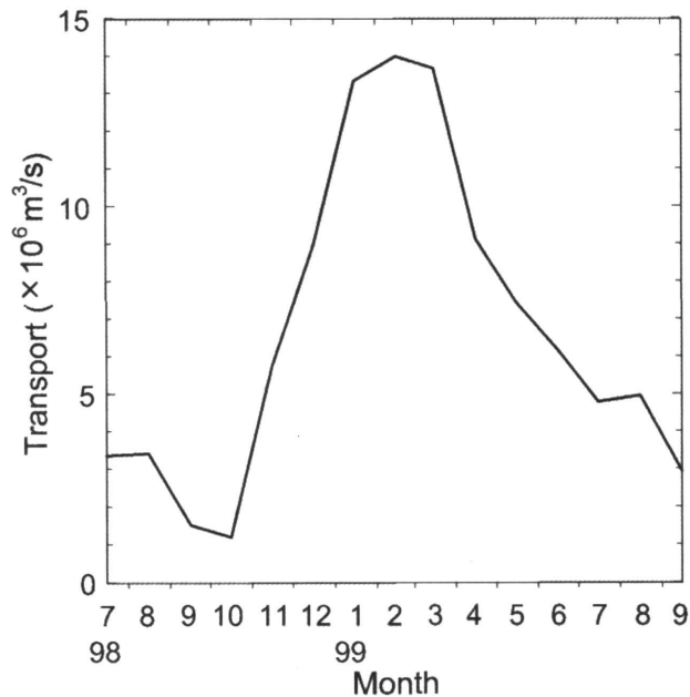
Figure 6: Seasonal variation of the ESC transport observed by moorings at 53^\circ\text{N} . Southward transport is taken positive. (Mizuta et al., 2003)
